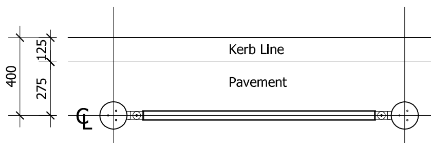
TYPICAL BARRIER OFFSET DETAIL @1:20
