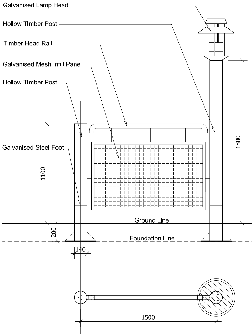
TYPICAL BARRIER & LAMP POST DETAIL @ 1:20
