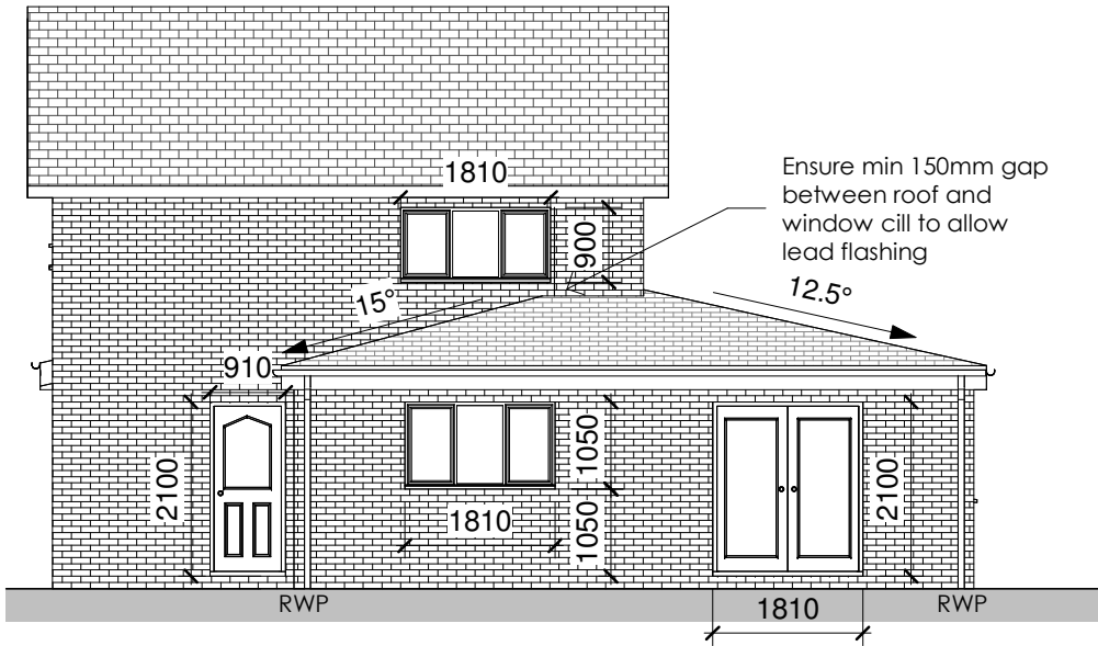
Rear Elevation 1 : 100
