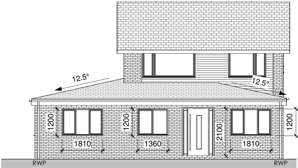
Front Elevation 1 : 100
