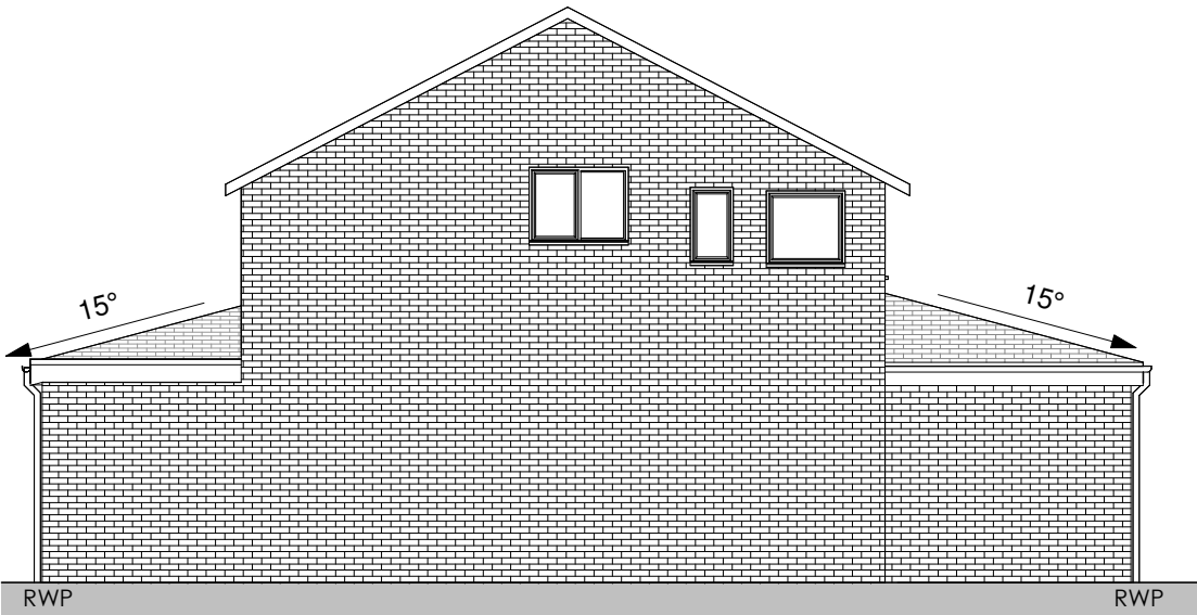
Side Elevation 1 : 100
