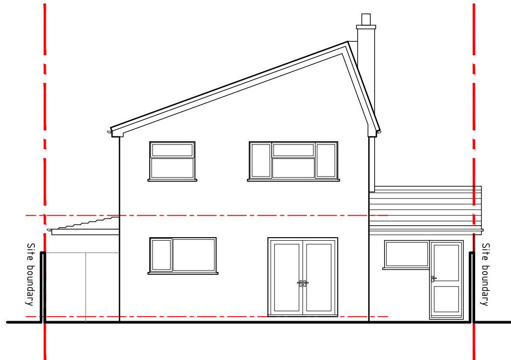
Rear elevation 1:100
