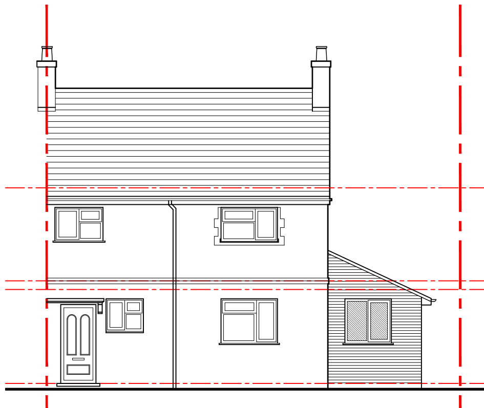
Front elevation 1:100
