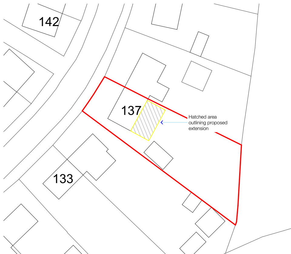
1 Site Block Plan 1:500
