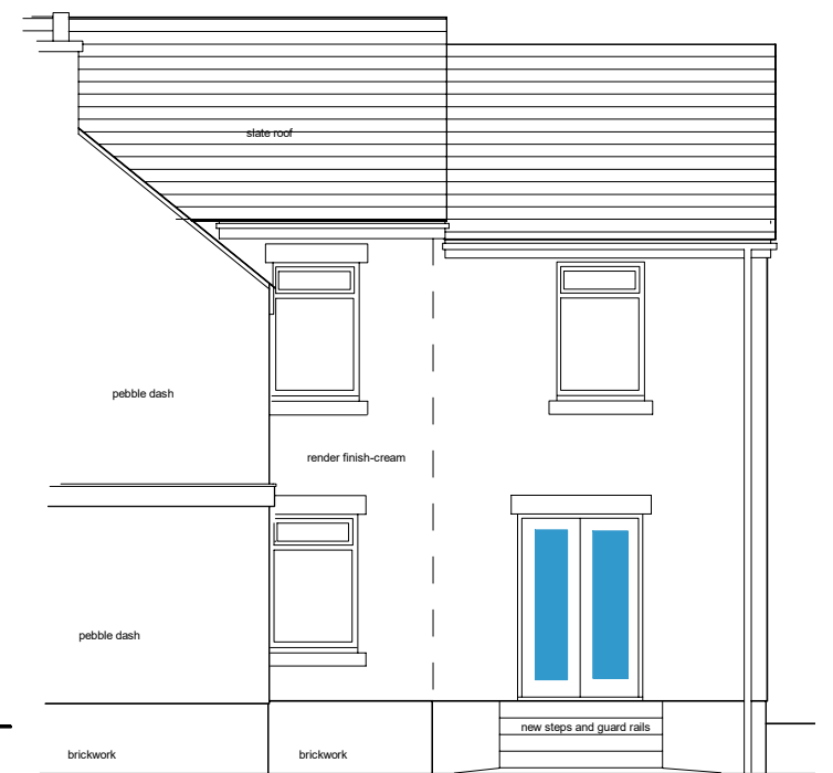
NORTH ELEVATION REAR
