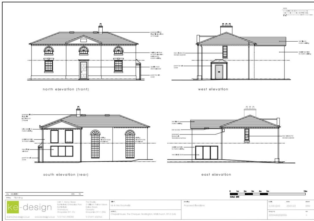
Fig.5: Proposed elevations.
