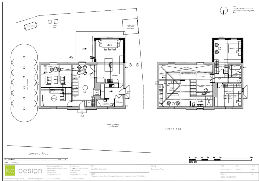
Fig.6: Proposed plans.
