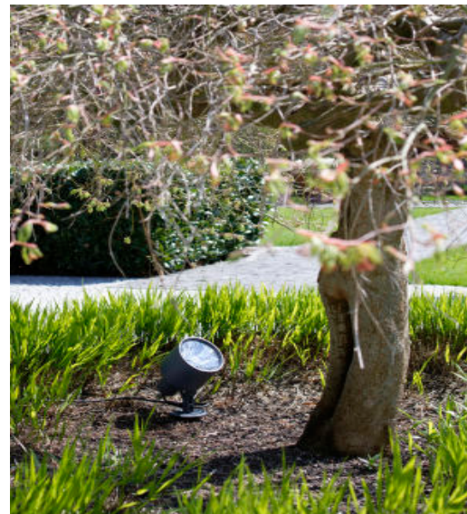
Proposed Tree Uplight (L4) Product: 84770 K3 (BEGA or similar approved) Dimensions: 135x200x230 Material: Cast aluminium, aluminium and S.S. Colour: Graphite
