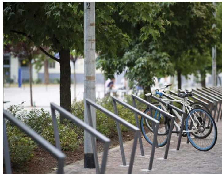
Proposed Cycle Stands (F5) Product: mMCite STE410 - Edgetyre (or similar approved) Dimensions: 965 x 885 x 50 mm Material: Steel
