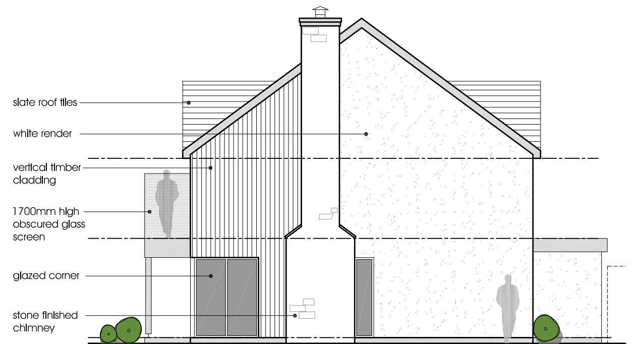
East Elevation (Side 1)
