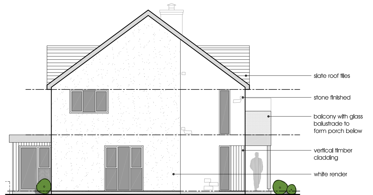
West Elevation (Side 2)
