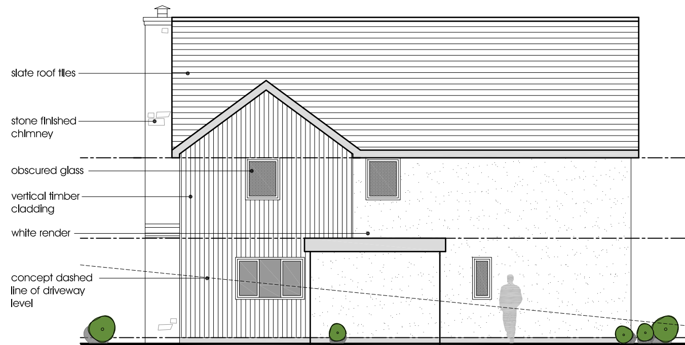
North Elevation (Front)
