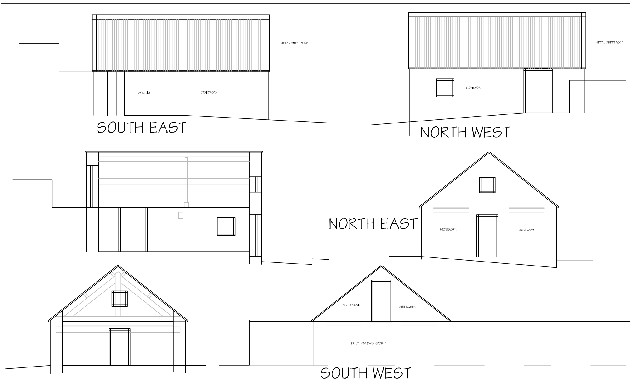
Figure 05: Existing elevations. Scale 1:100 at A4.
