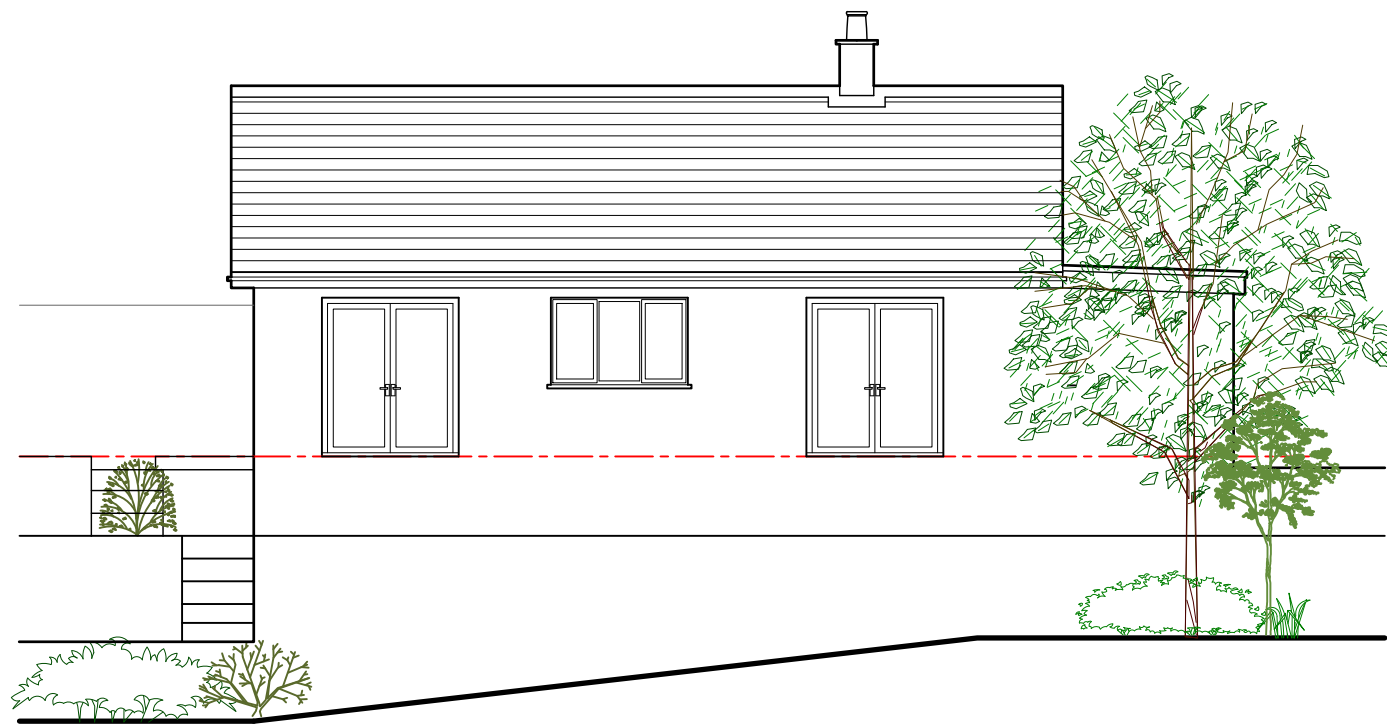
Front elevation 1:100
