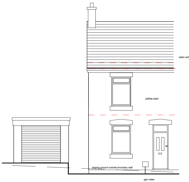
SOUTH ELEVATION FRONT
