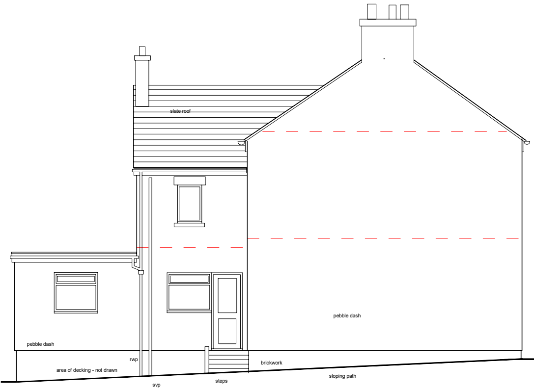
WEST ELEVATION GABLE
