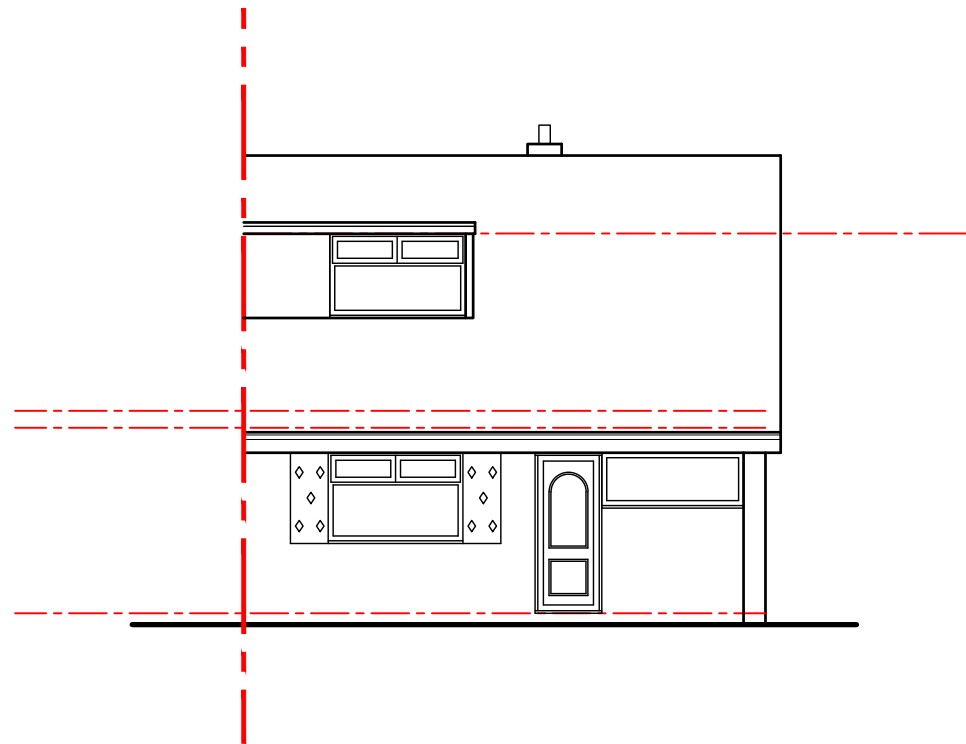
Front elevation 1:100
