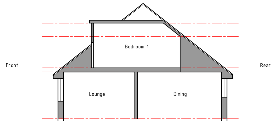
Typical Section 1:100
