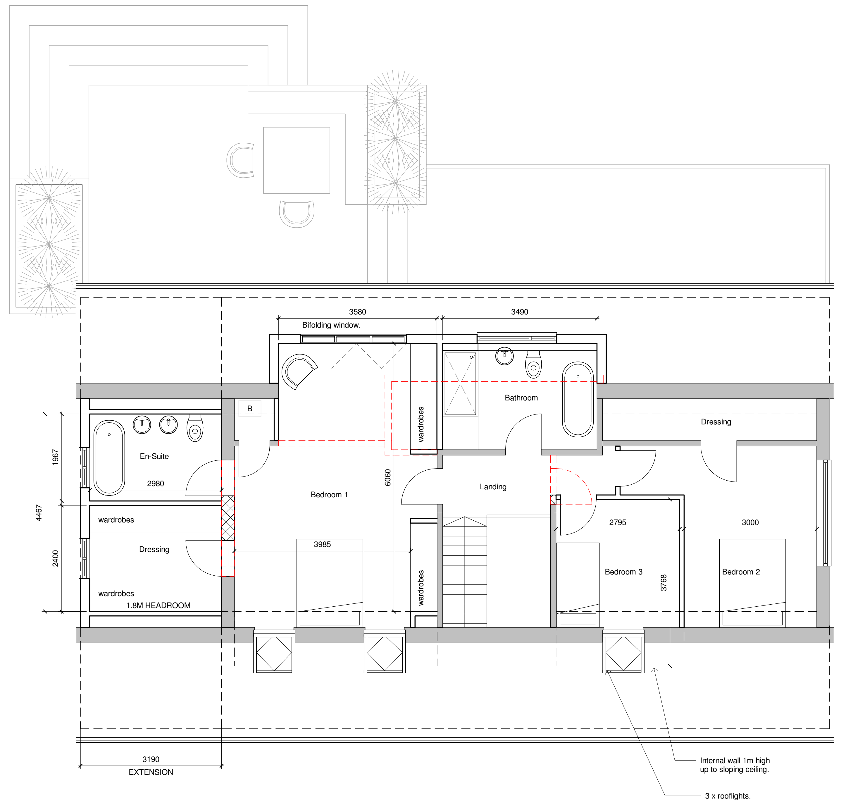
Proposed First Floor Plan 1 : 50
