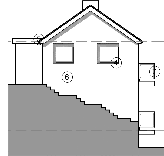
SIDE ELEVATION
