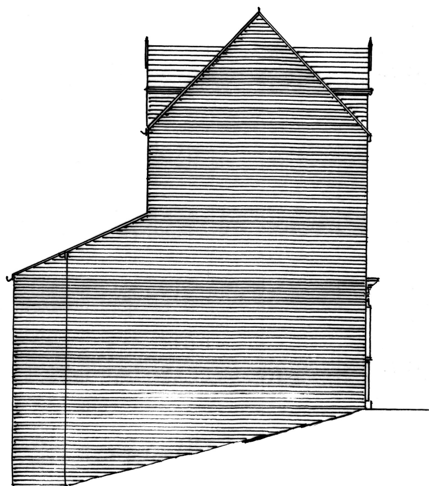
SIDE ELEVATION
