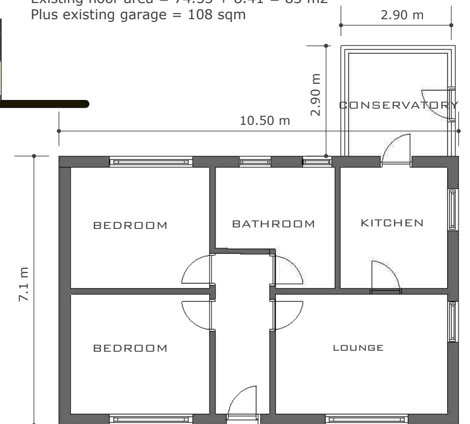
A 7 Floor Plan 1:100
