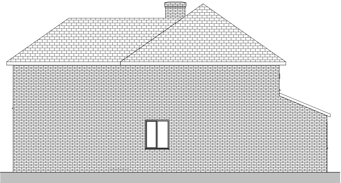
Side Elevation 2 1 : 100
