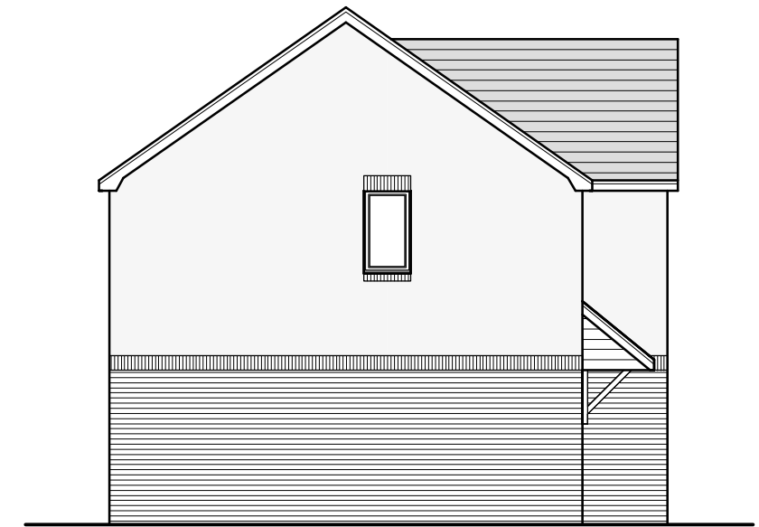
Side Elevation 1:100
