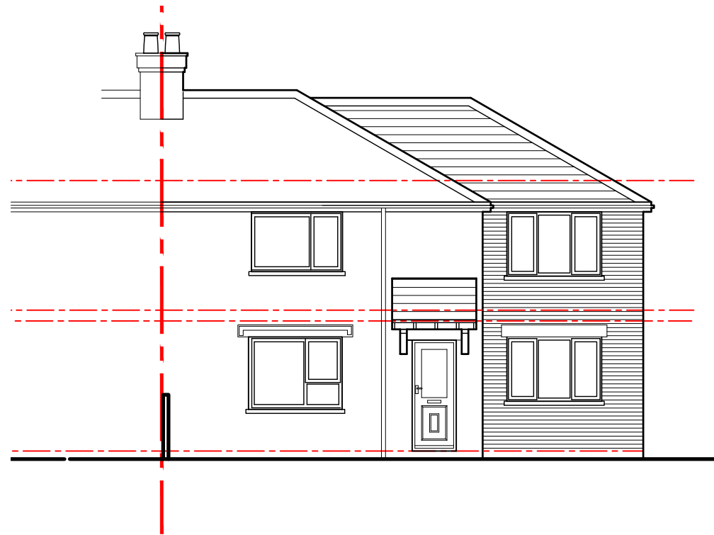
Front elevation 1:100
