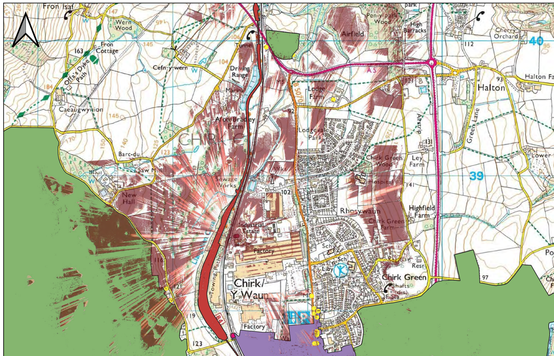
Figure 11. ZTV model - silos 24m height
