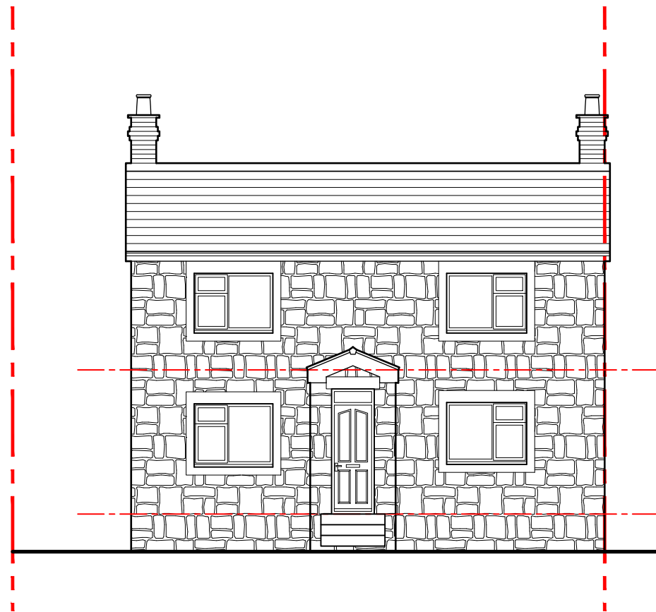
Front elevation 1:100
