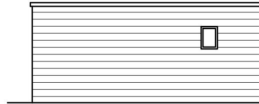
Rear Elevation
