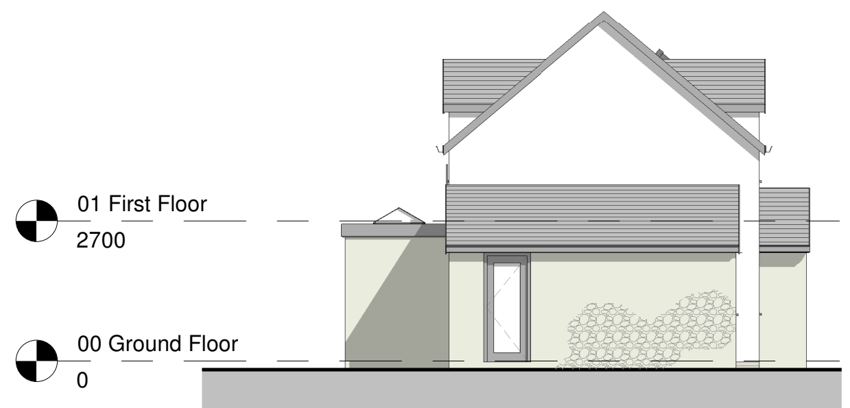
South Elevation 1 : 100
