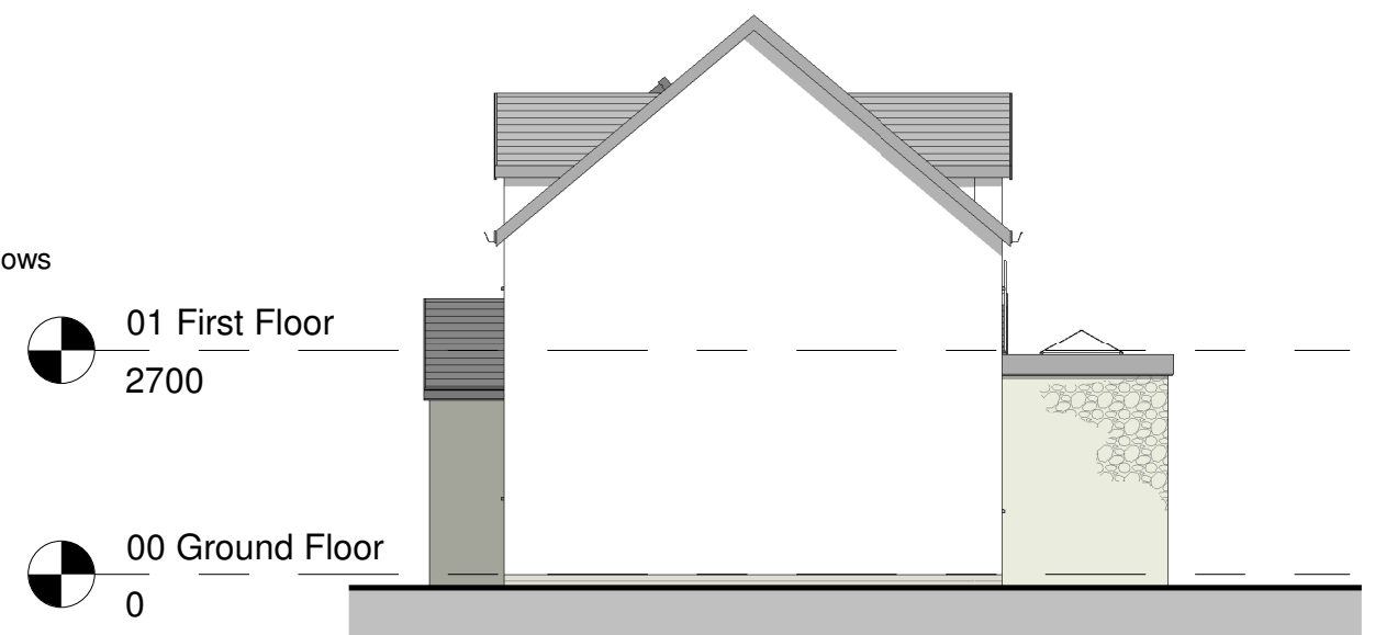
North Elevation 1 : 100
