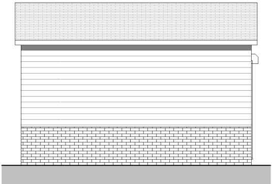
Side Elevation 1 : 100
