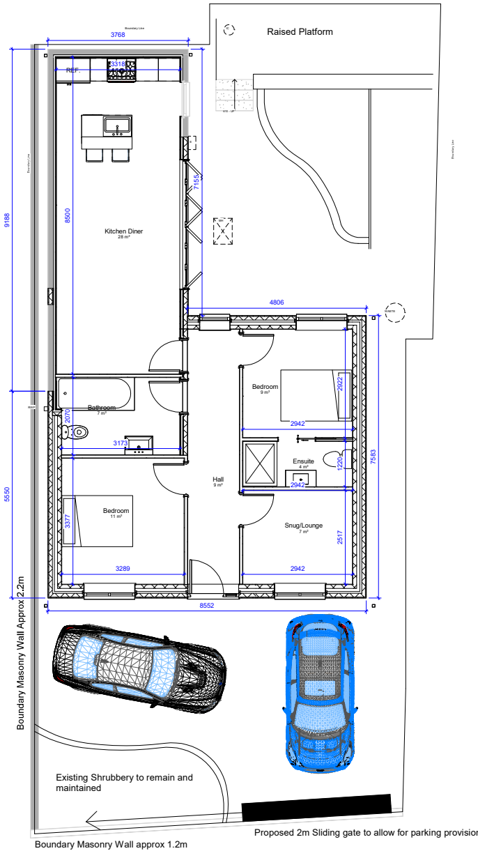
**1 Proposed Ground Level 1 : 50
