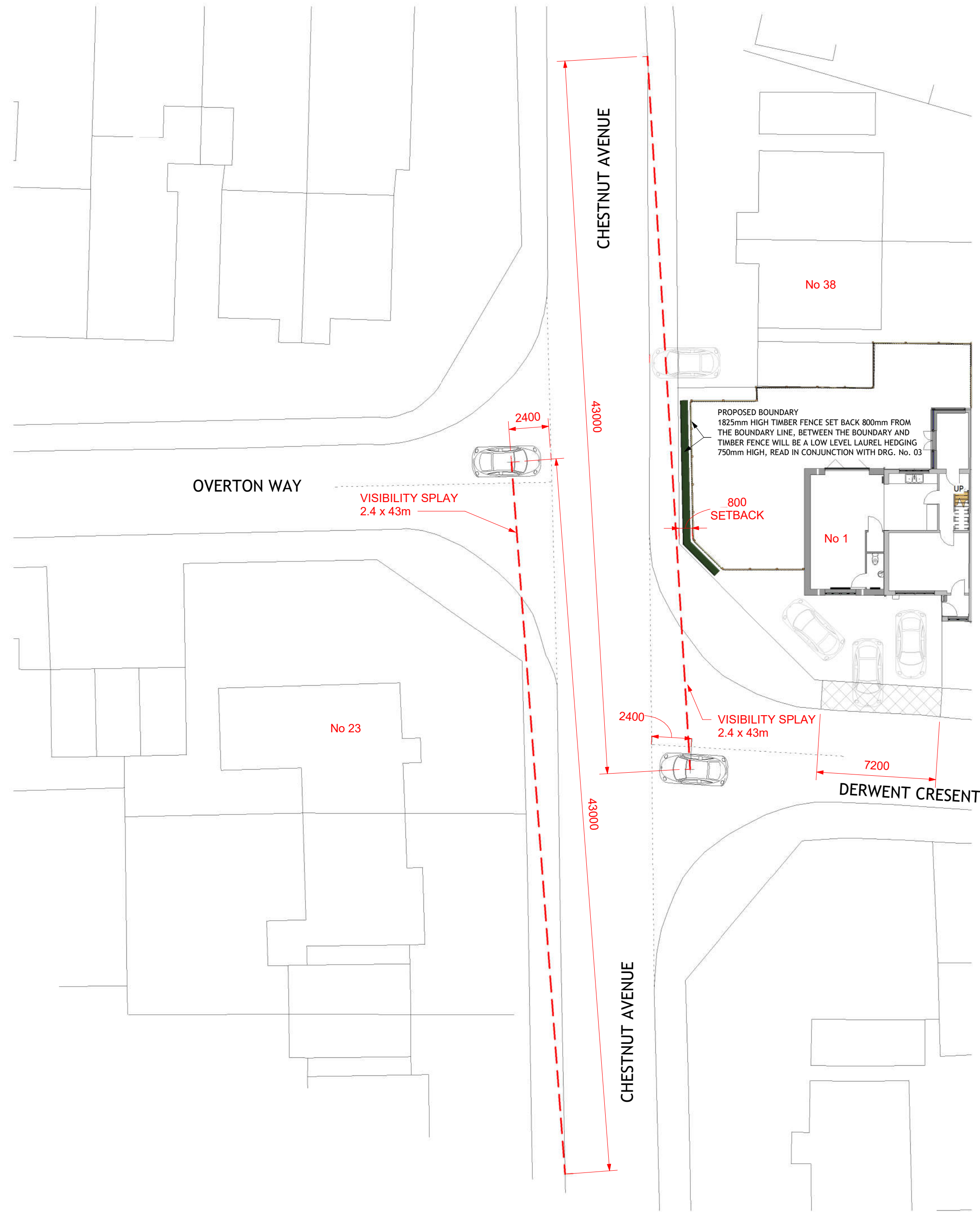
1 VISIBILITY SPLAYS - CHESTNUT AV. / DERWENT CRESENT & OVERTON WAY 1 : 200
