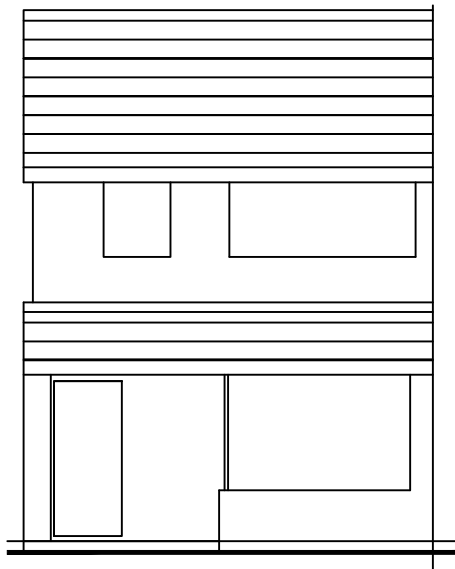
Front Elevation 1:100
