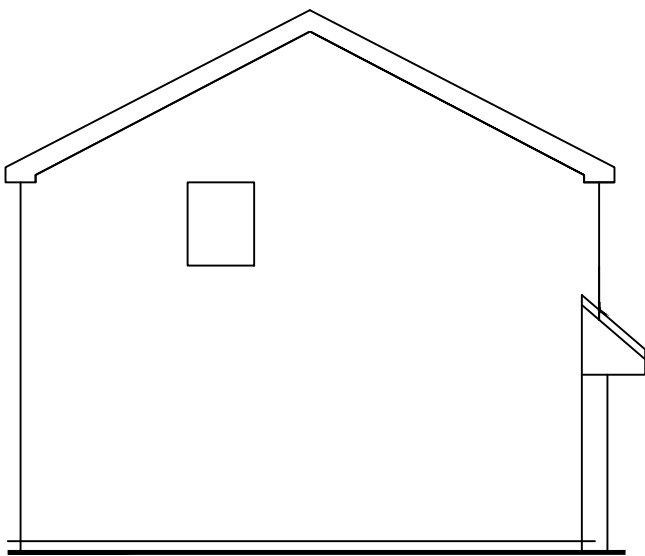
Side Elevation 1:100
