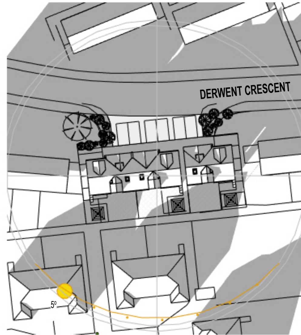
6 Dec 21 1500 1 : 500 Winter Solstice sunrise 08:04 sunset 15:53
