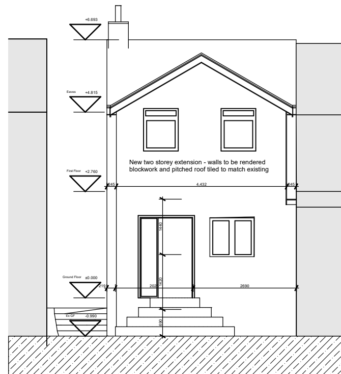
4 Rear Elevation - Proposed - 1:100
