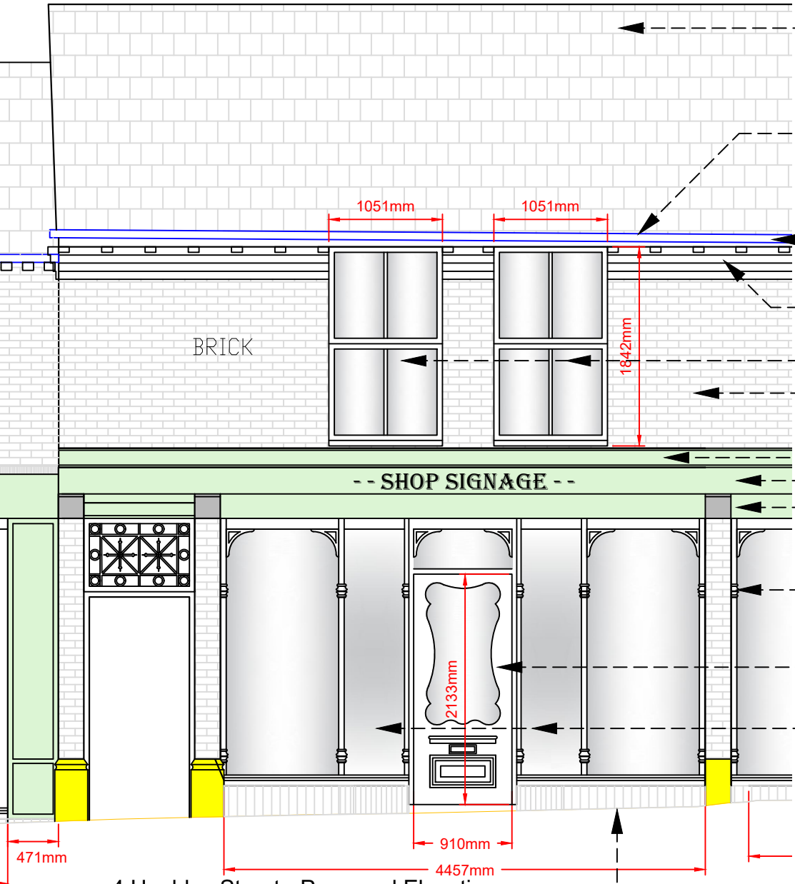
4 Henblas Street - Proposed Elevation
