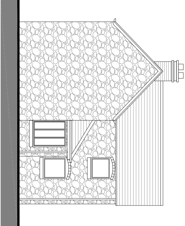
North/Side Elevation 1:100
