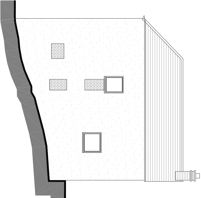
West/Rear Elevation 1:100
