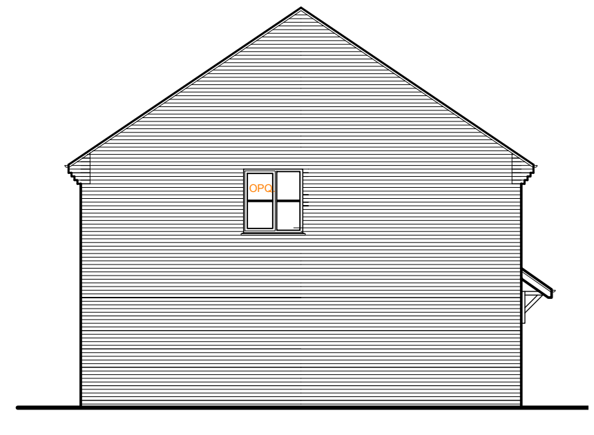
4 SIDE ELEVATION (EAST)
