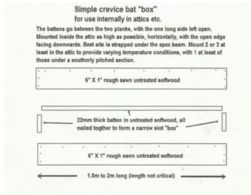
Figure 13: Simple crevice boxes design.
