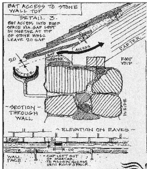
Figure 9: Bat access via eaves
