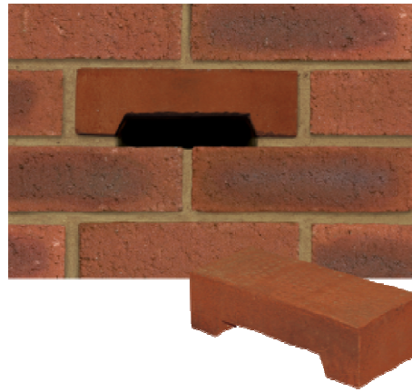
Figure 8: Istock type bat brick.
