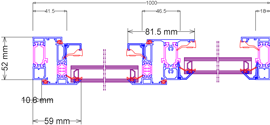
Horizontal section A-A (1:2)
