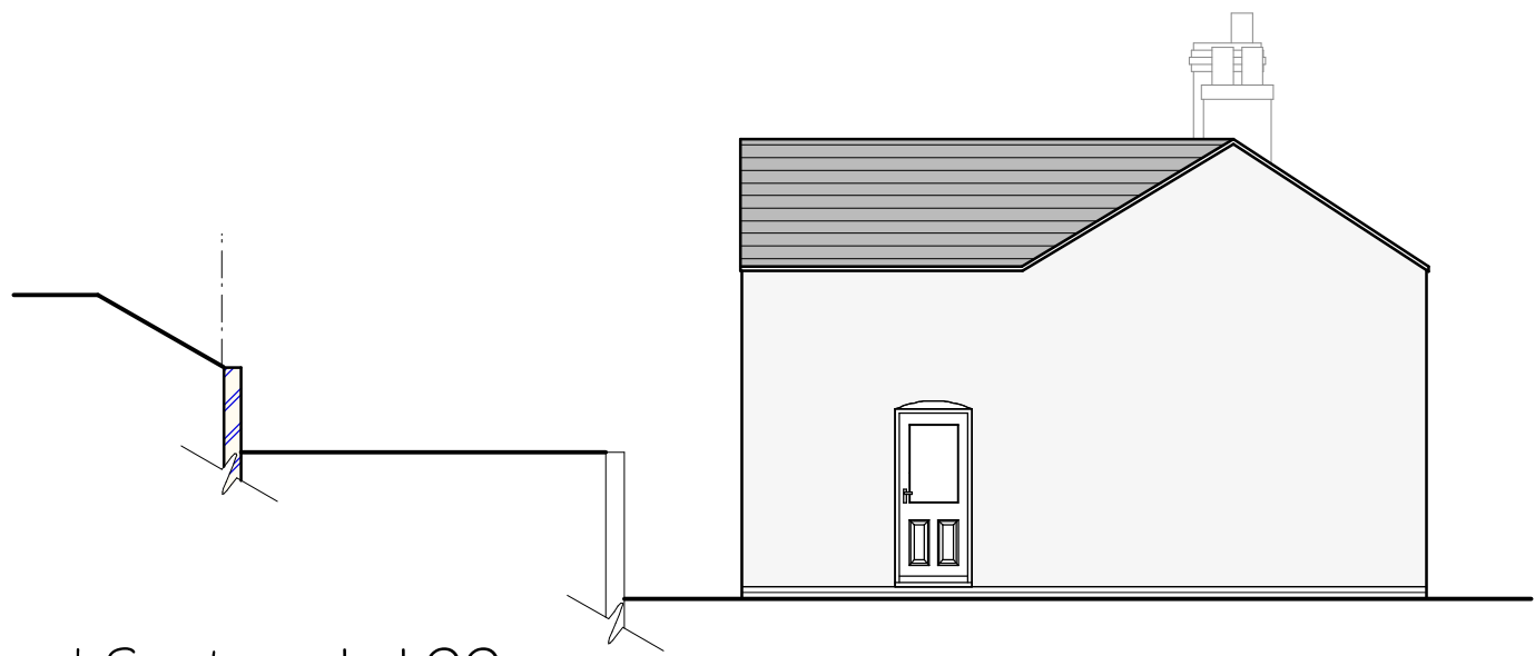
Typical Section 1:100
