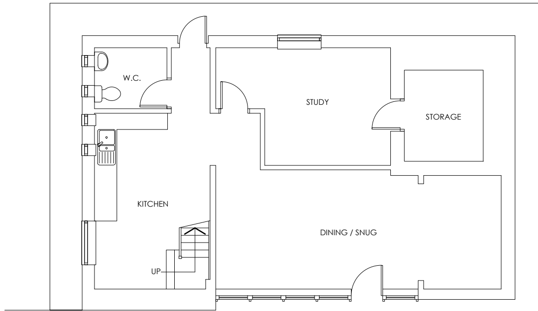
GROUND PLAN
