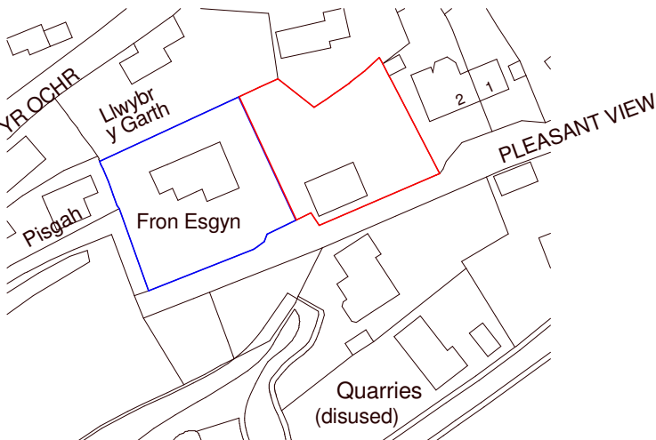
Location Plan 1 : 1250
