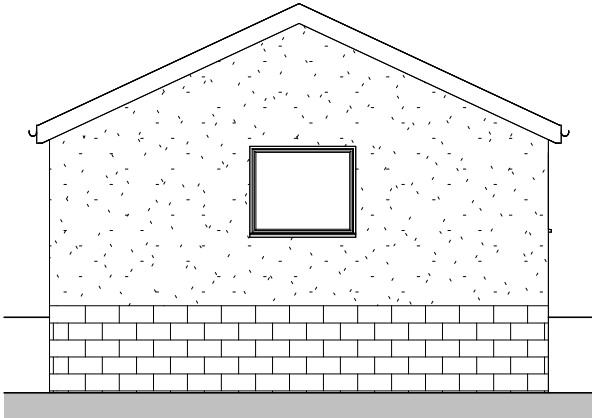
Rear Elevation 1 : 100
