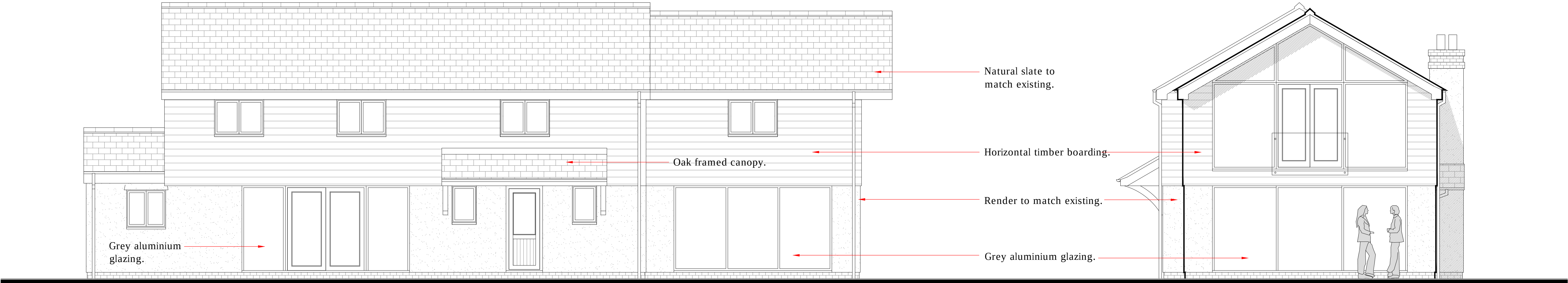
Proposed Front Elevation 1:100
