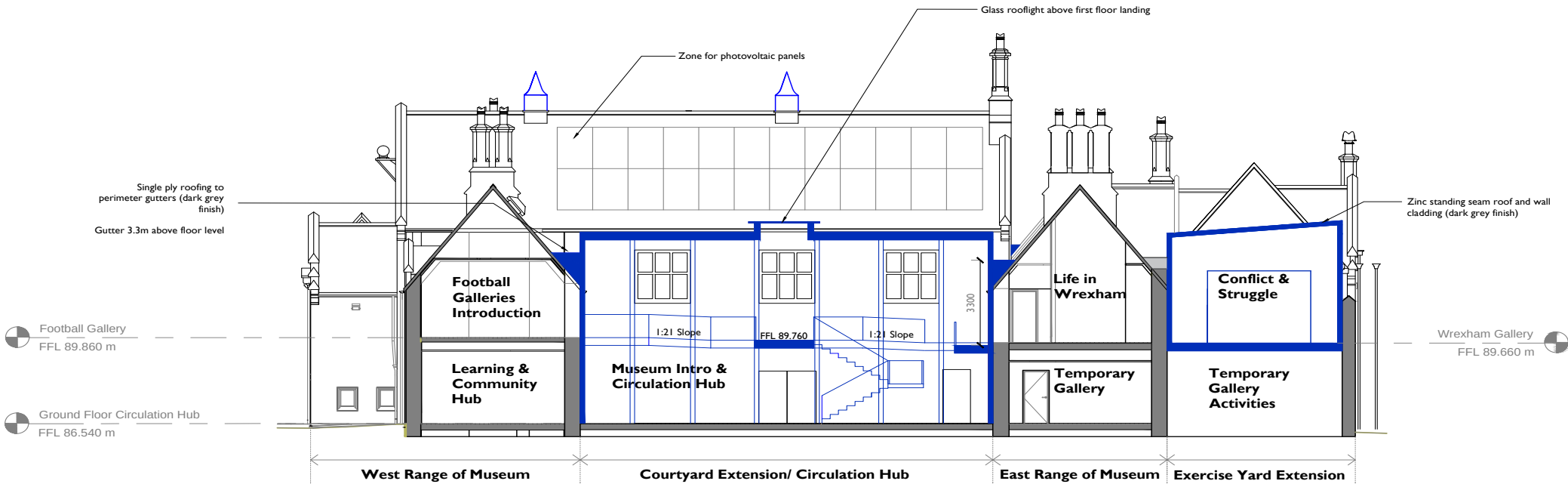
Section 1 Proposed
