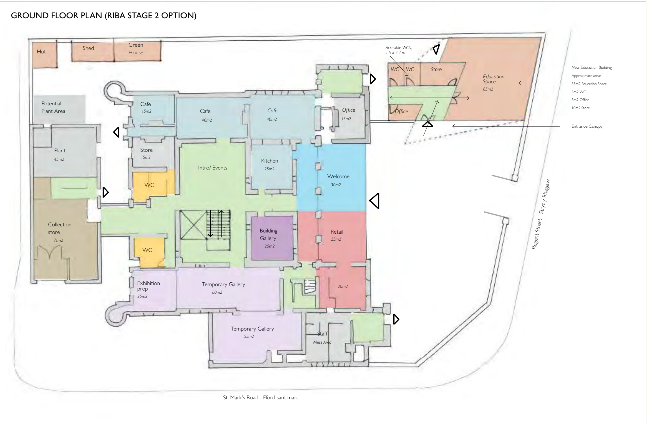
RIBA Stage 2 Preferred Option: Ground Floor
