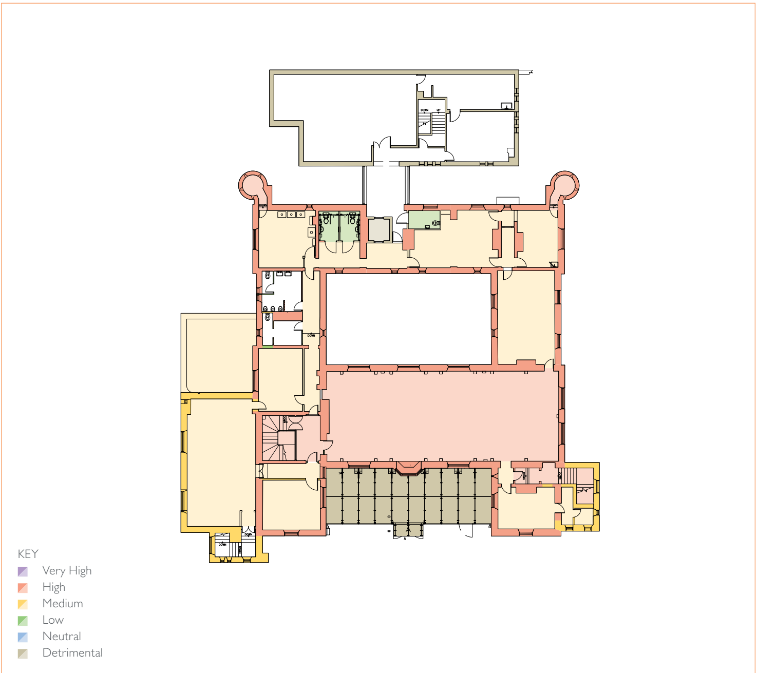
First Floor Significance Plan
