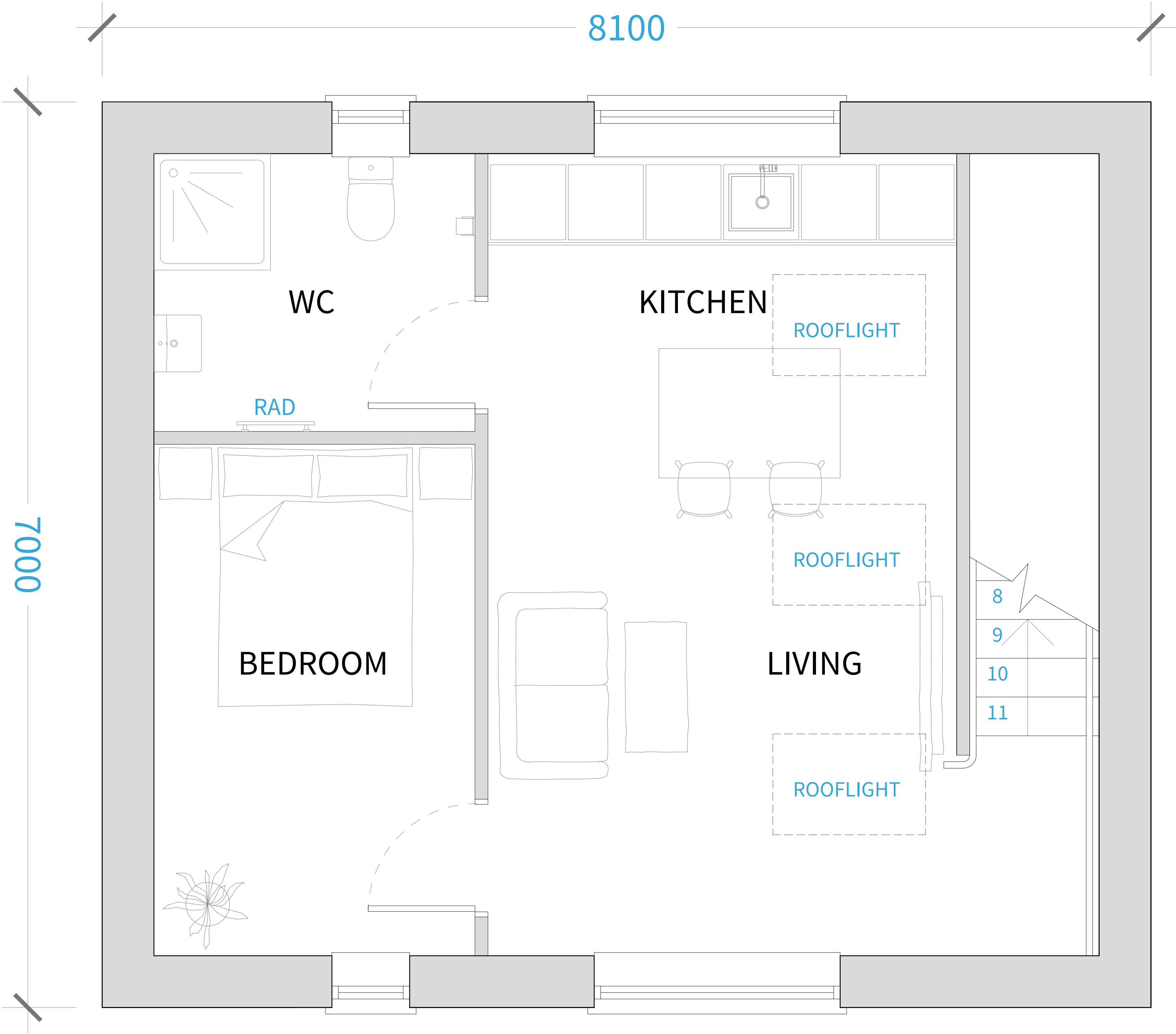
PROPOSED FIRST FLOOR (1:20)
