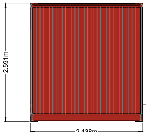
NORTHERN ELEVATION
