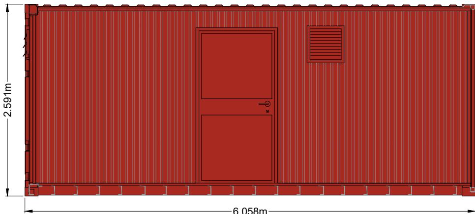
WESTERN ELEVATION
