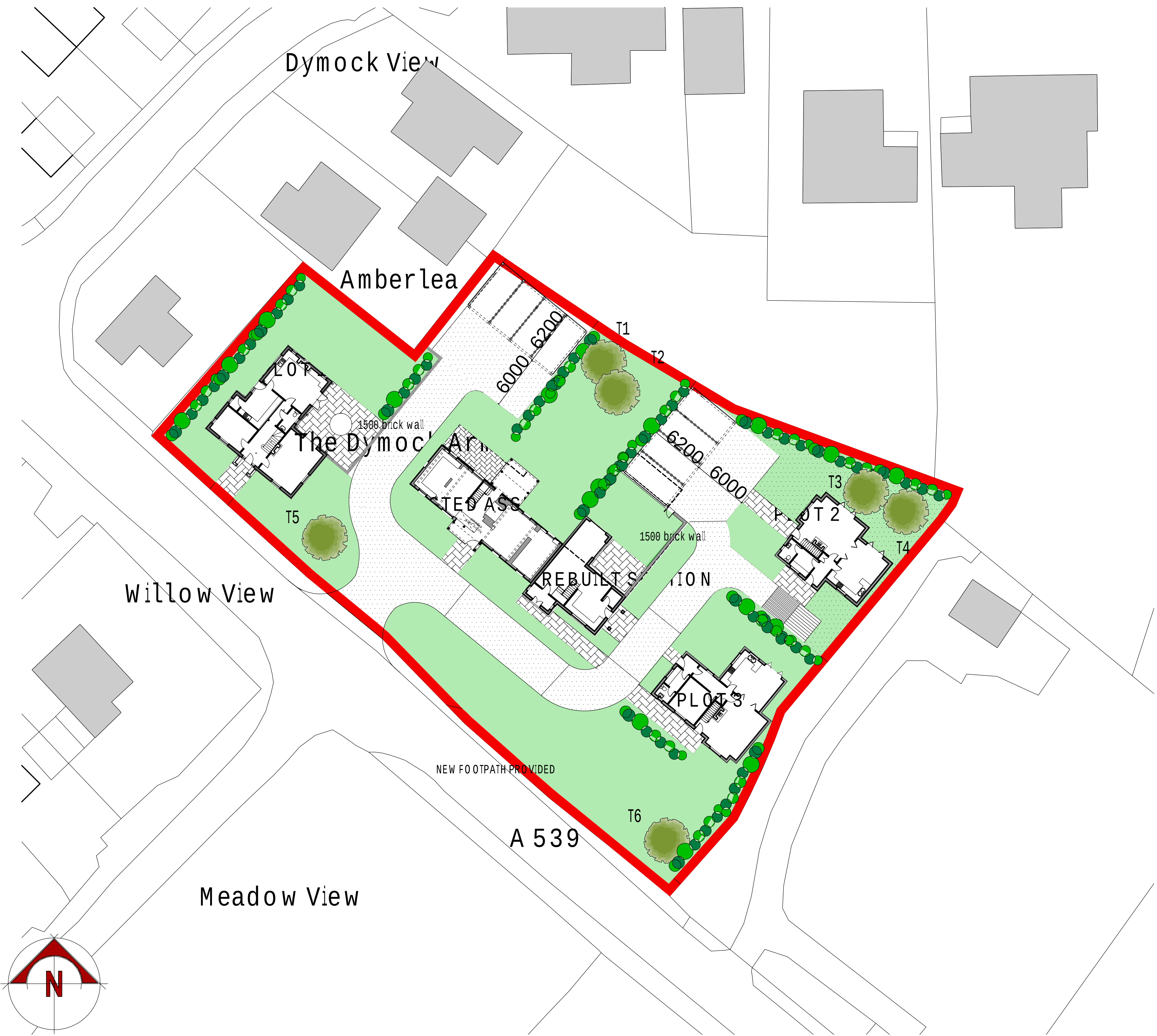
1800 CLOSE BOARDED FENCE to site boundary
