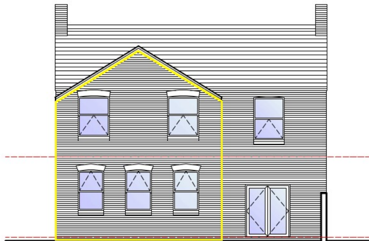
REAR ELEVATION
