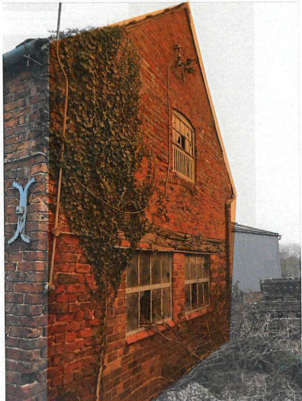
SOUTH GABLE IS SIGNIFICANTLY DISTORTED, NUMEROUS BRICKS ARE WEATHERED AND THE TIMBER WITHIN THE WALL IS SUBJECT TO ONGOING DECAY. PREFERABLE TO DEMOLISH AND REBUILD
