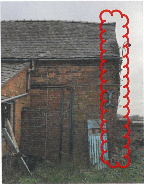
SOUTH GABLE IS SIGNIFICANTLY DISTORTED, NUMEROUS BRICKS ARE WEATHERED AND THE TIMBER WITHIN THE WALL IS SUBJECT TO ONGOING DECAY. PREFERABLE TO DEMOLISH AND REBUILD
