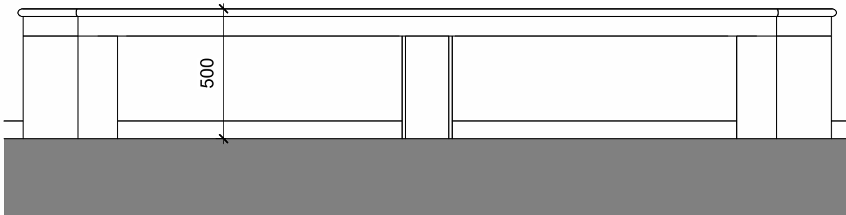
Besoke Stone Bench - Elevation 1 : 20
