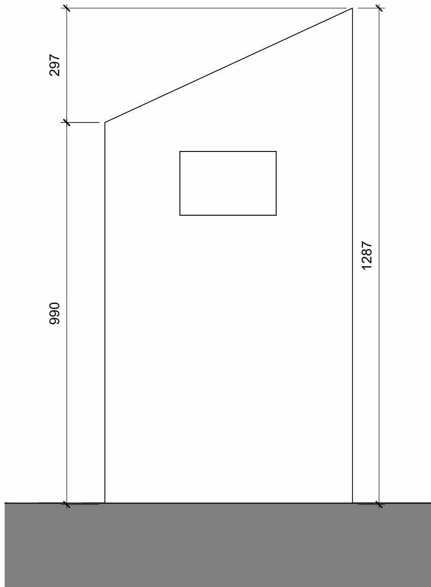
Bespoke Stone Memorial - Elevation 1 : 10
