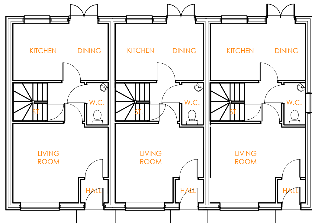
1 GROUND FLOOR
