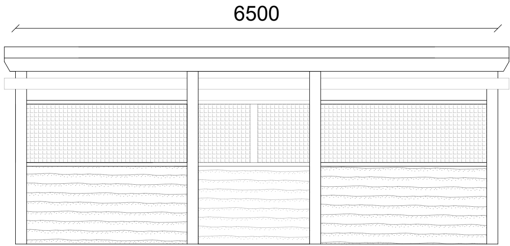
EAST ELEVATION @ 1:50
