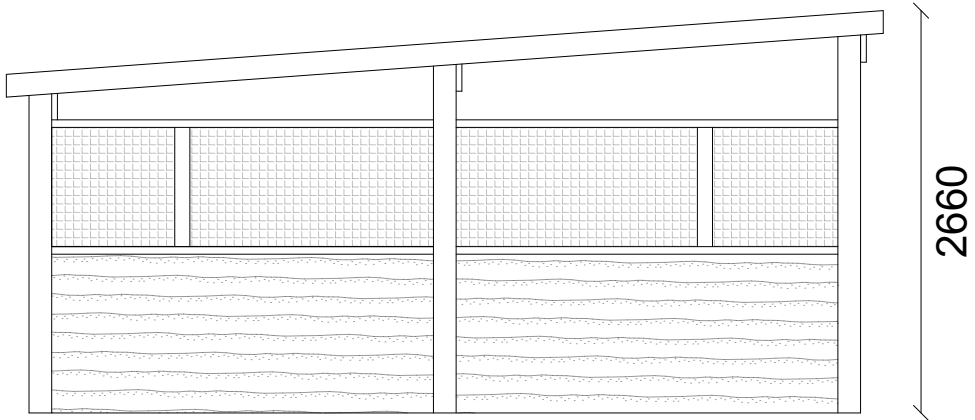
SOUTH ELEVATION @ 1:50
