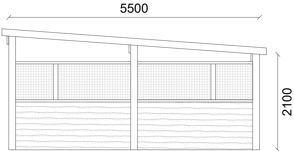
NORTH ELEVATION @ 1:50
