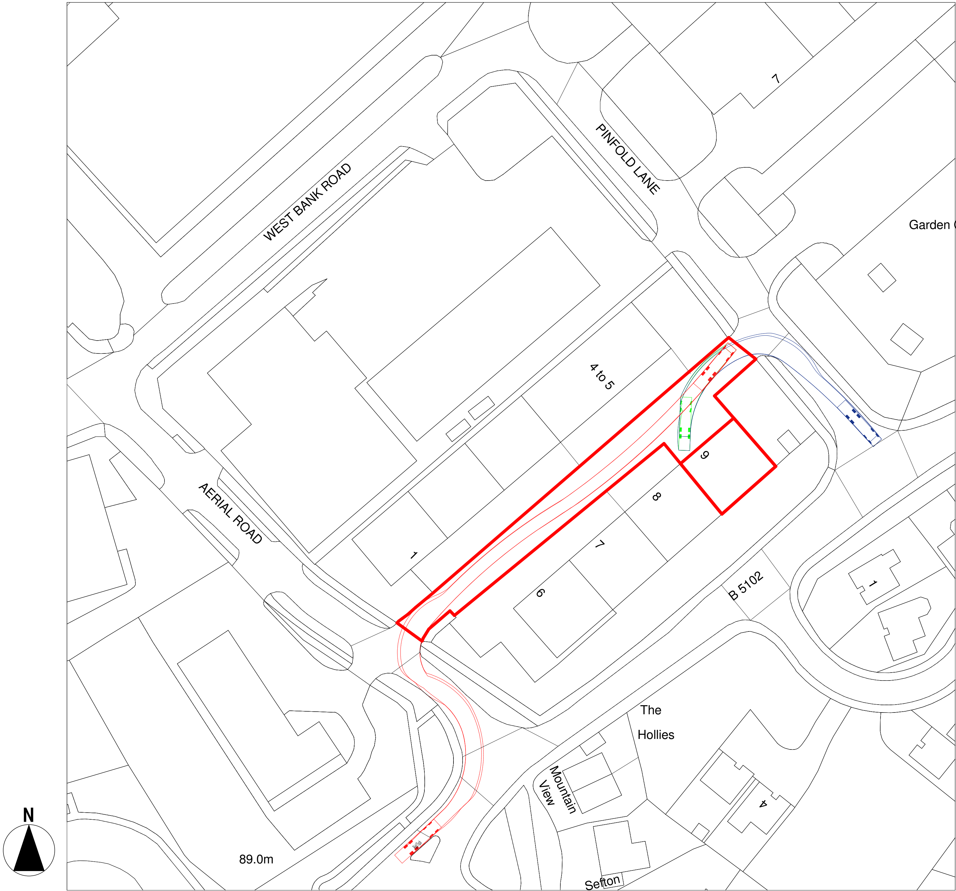
PROPOSED VEHICLE TRACKING PLAN SCALE 1 : 500
