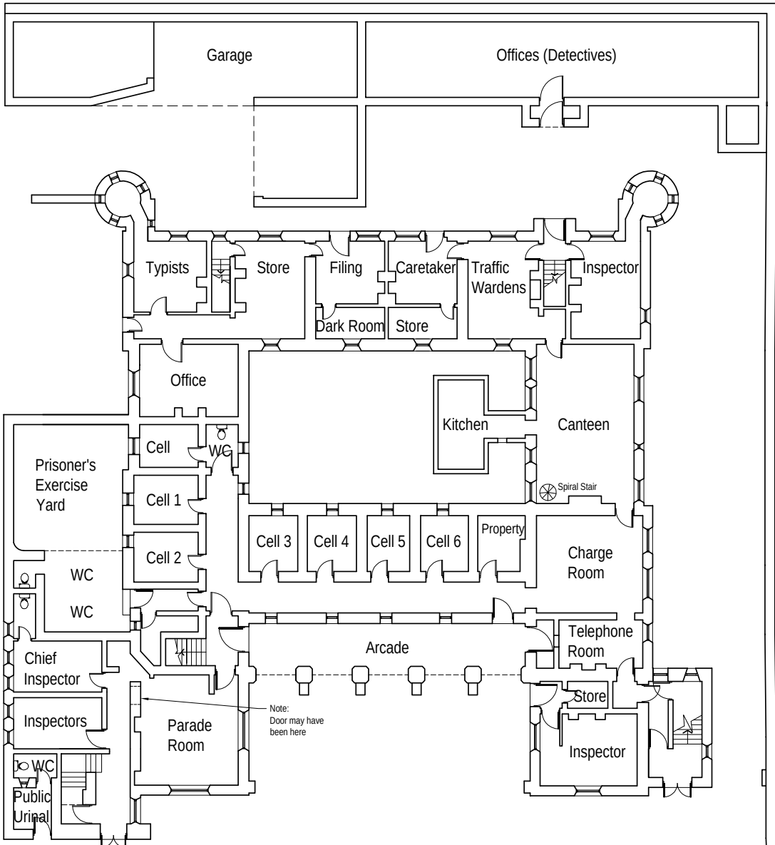
1967 Ground Floor Plan
