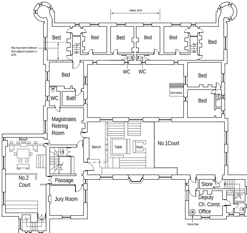
1896 First Floor Plan
