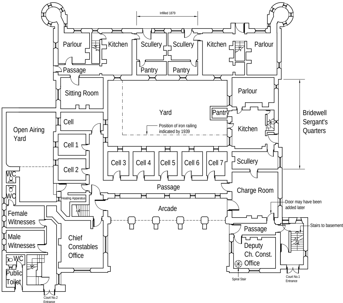
1896 Ground Floor Plan
