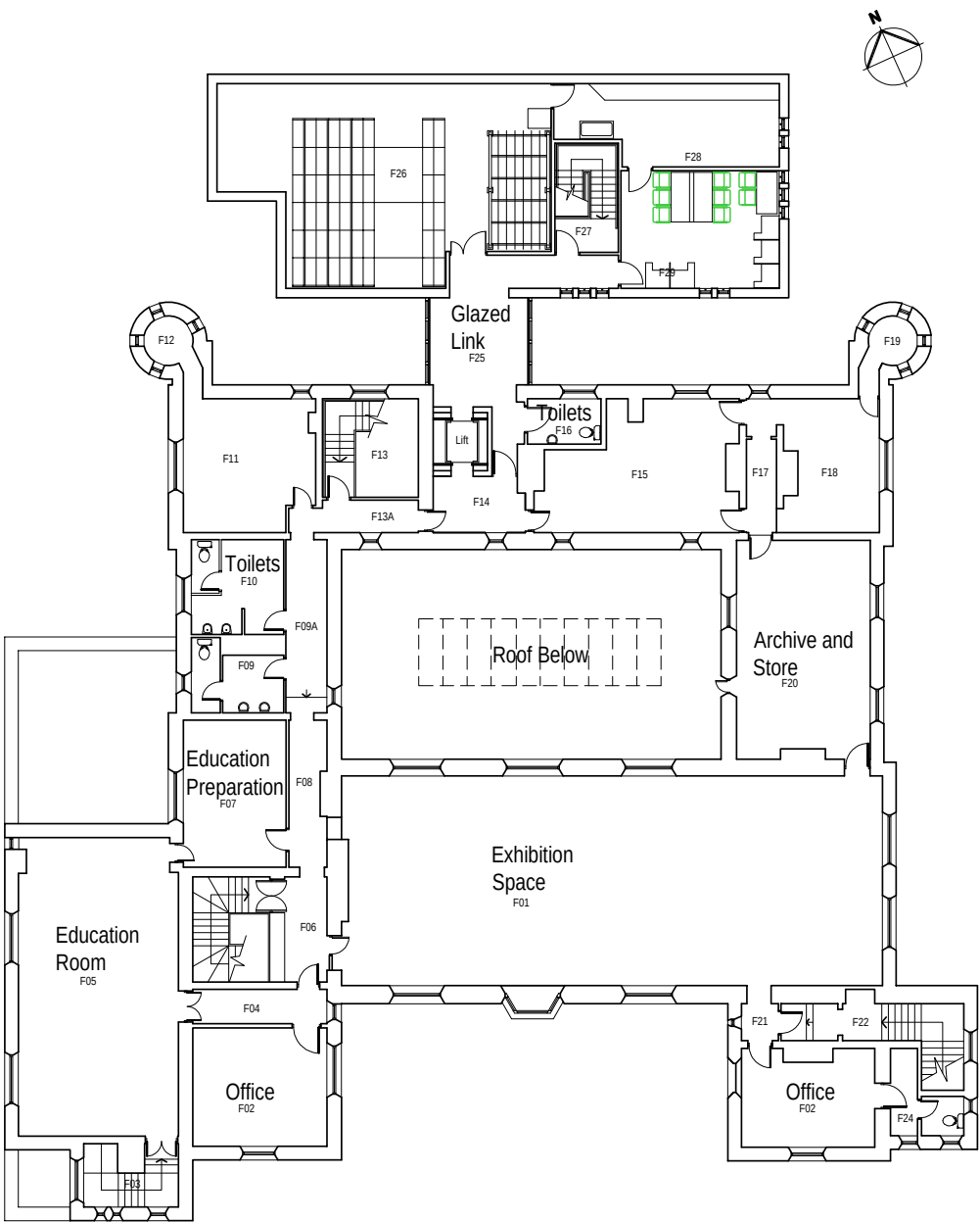
First Floor Plan 2005
